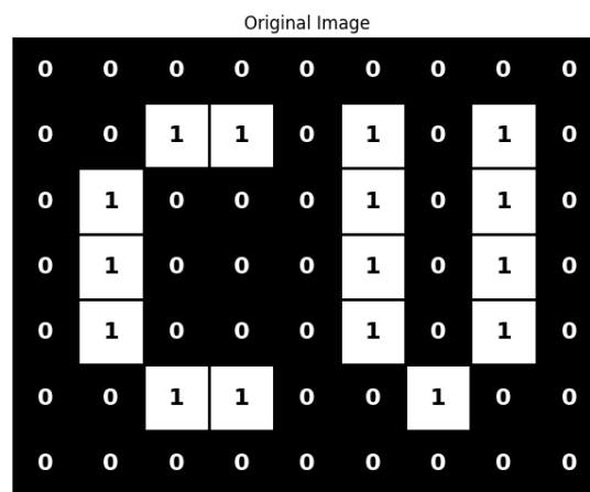
Figure 7: A binary image for connected component analysis.
