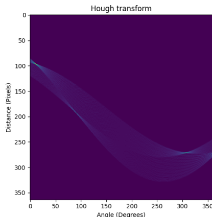
Figure 9: The accumulator matrix depicted as an image. This matrix results from applying a Hough Transform to an image with lines.
